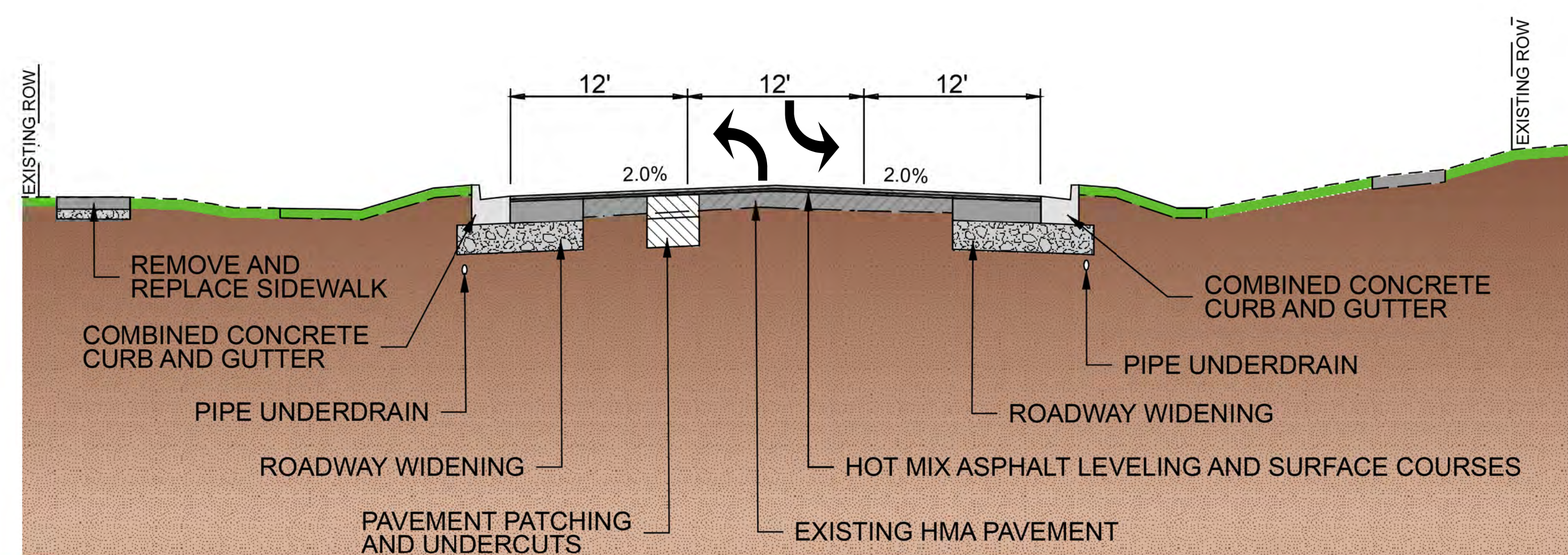
FINAL TYPICAL SECTION EAST OF 7TH STREET
