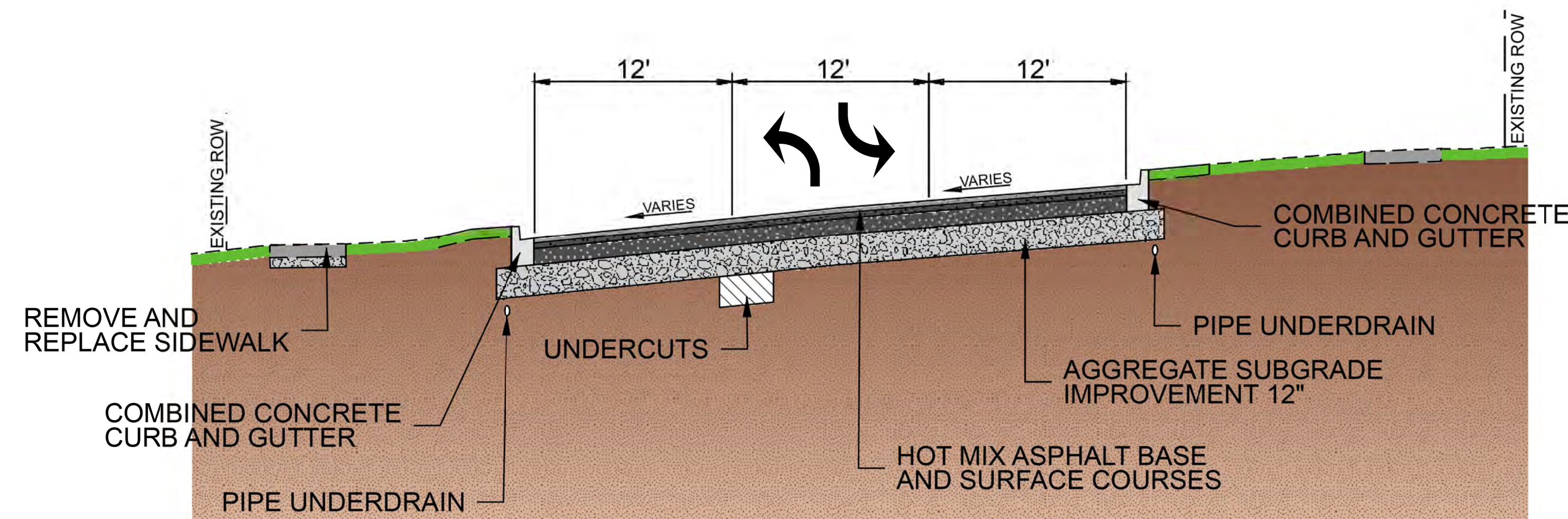
FINAL TYPICAL SECTION WEST OF 7TH STREET
